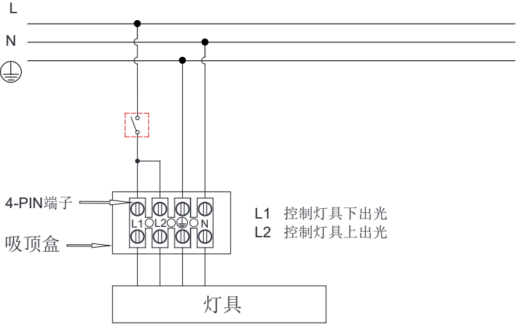
上出光和下出光统一开关(ON/OFF)功能
