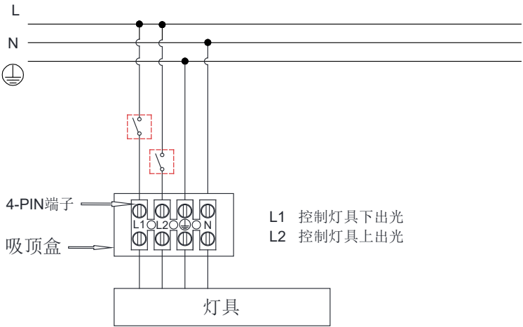
上出光和下出光独立开关(ON/OFF)功能
